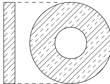
PISTON BUMPER P/N 11-5051P000 REPLACES P/N 10-450-51 QTY: 1
